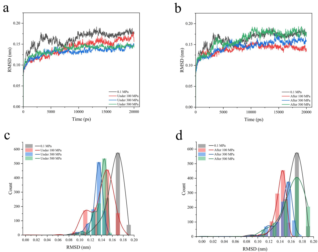
Fig. S1 RMSD of PPO systems during the pressurization and depressurization stages from MD simulations. RMSD plots of 0.1 MPa, under 100 MPa, under 300MPa, and under 500MPa (a); 0.1 MPa, after 100 MPa, after 300 MPa, after 500 MPa (b). RMSD Histograms of 0.1 MPa, under 100 MPa, under 300MPa, and under 500MPa (c); 0.1 MPa, after 100 MPa, after 300 MPa, after 500 MPa (d).
