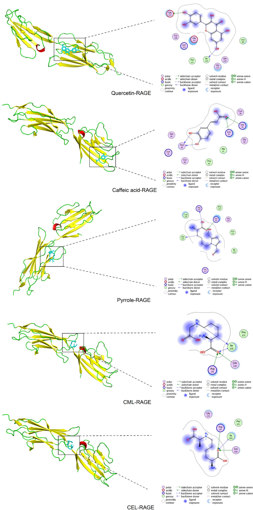
Fig. S12 Analysis of the interaction between quercetin, caffeic acid, pyrrole, CML, CEL and RAGE
