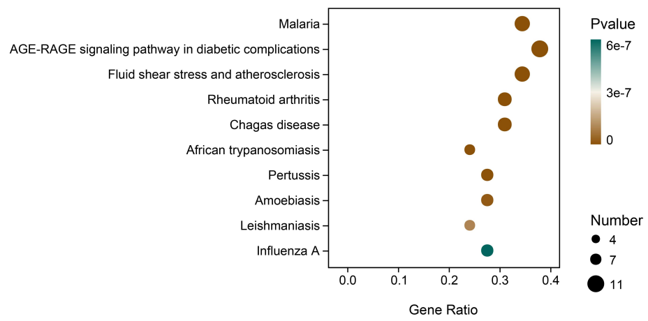
Fig. S5 KEGG enrichment analysis plot
