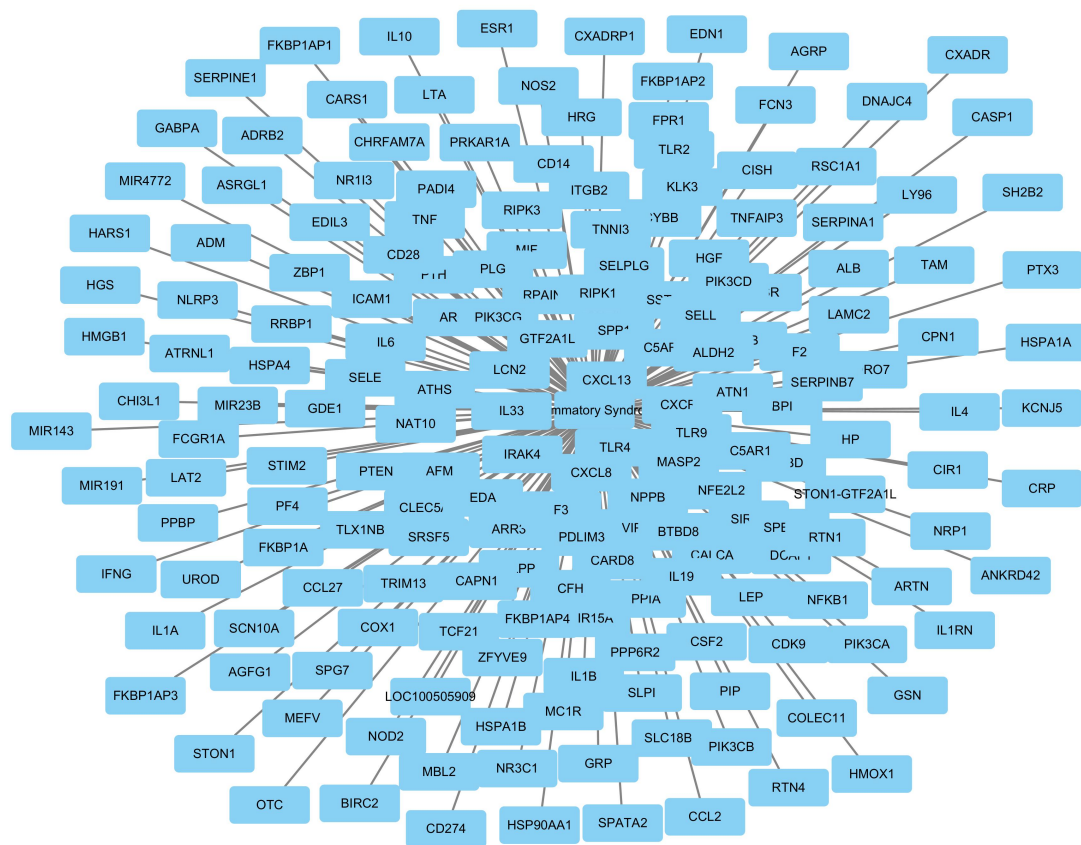
Fig. S2 Inflammation-target network relationships
