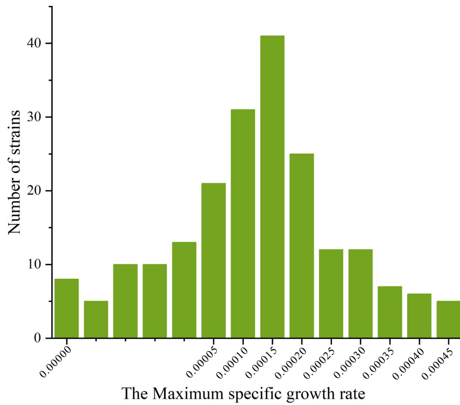
Fig. S4 Histogram of the maximum specific growth rate of the haploid.
