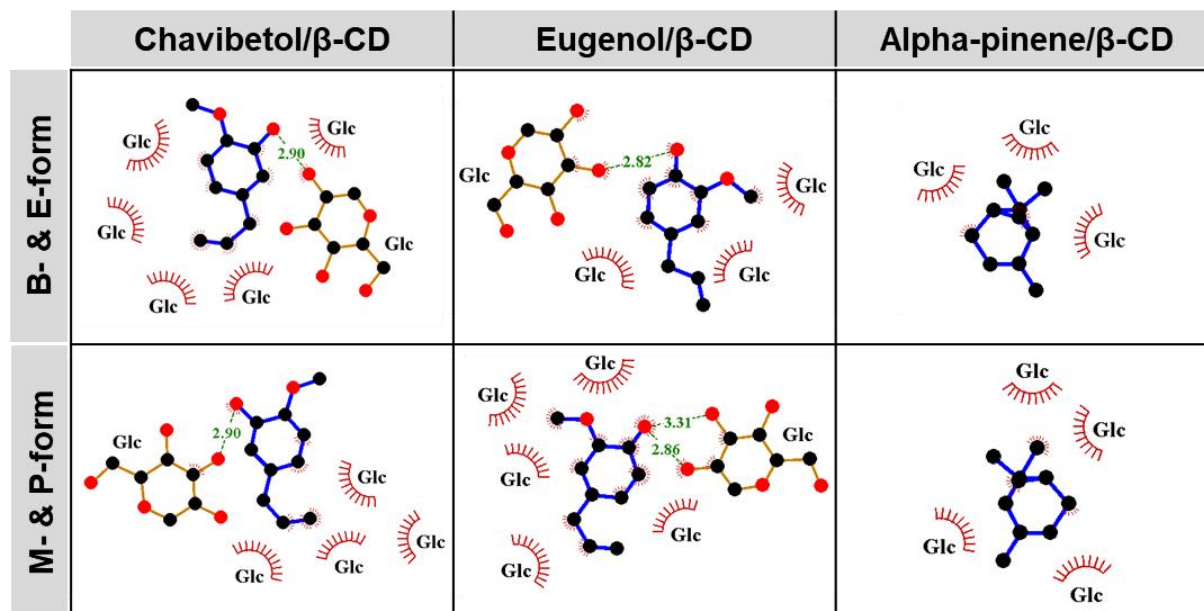
Supplementary Fig. S15. The 2D guest–host interactions of all studied ICs in both orientations (B- & E-form and M- & P-form). Glc represents the glucopyranose unit.
