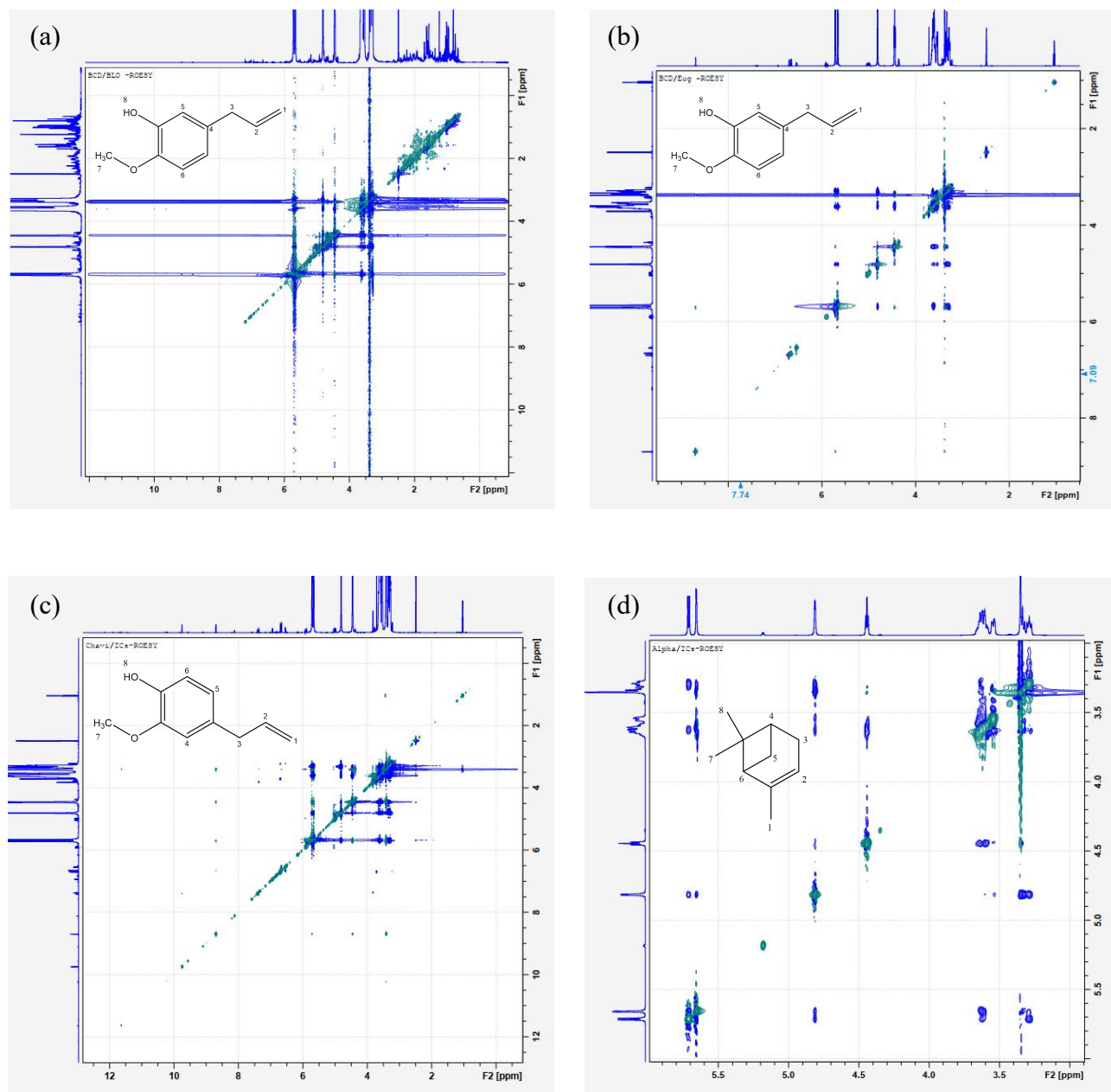
Supplementary Fig. S5. 2D ROESY NMR spectra of a) BLO/ \beta -CD, b) chavibetol/ \beta -CD, c) eugenol/ \beta -CD, and d) \alpha -pinene/ \beta -CD.
