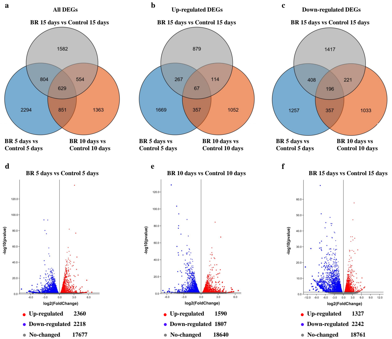
Figure S2 Venn diagrams and volcano plots displaying the numbers of differentially expressed genes (DEGs) in 2,4-epibrassinolide (EBR) treated berries, according to the developmental stage. DEGs were screened by |\log_2(\text{Fold change})| > 1 and an adjusted P < 0.05 (with FDR correction).
