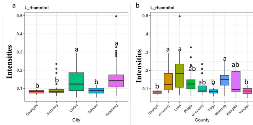
Figure S5. Quantification of L-rhamnitol in different locations at the city (a) and county level (b).
