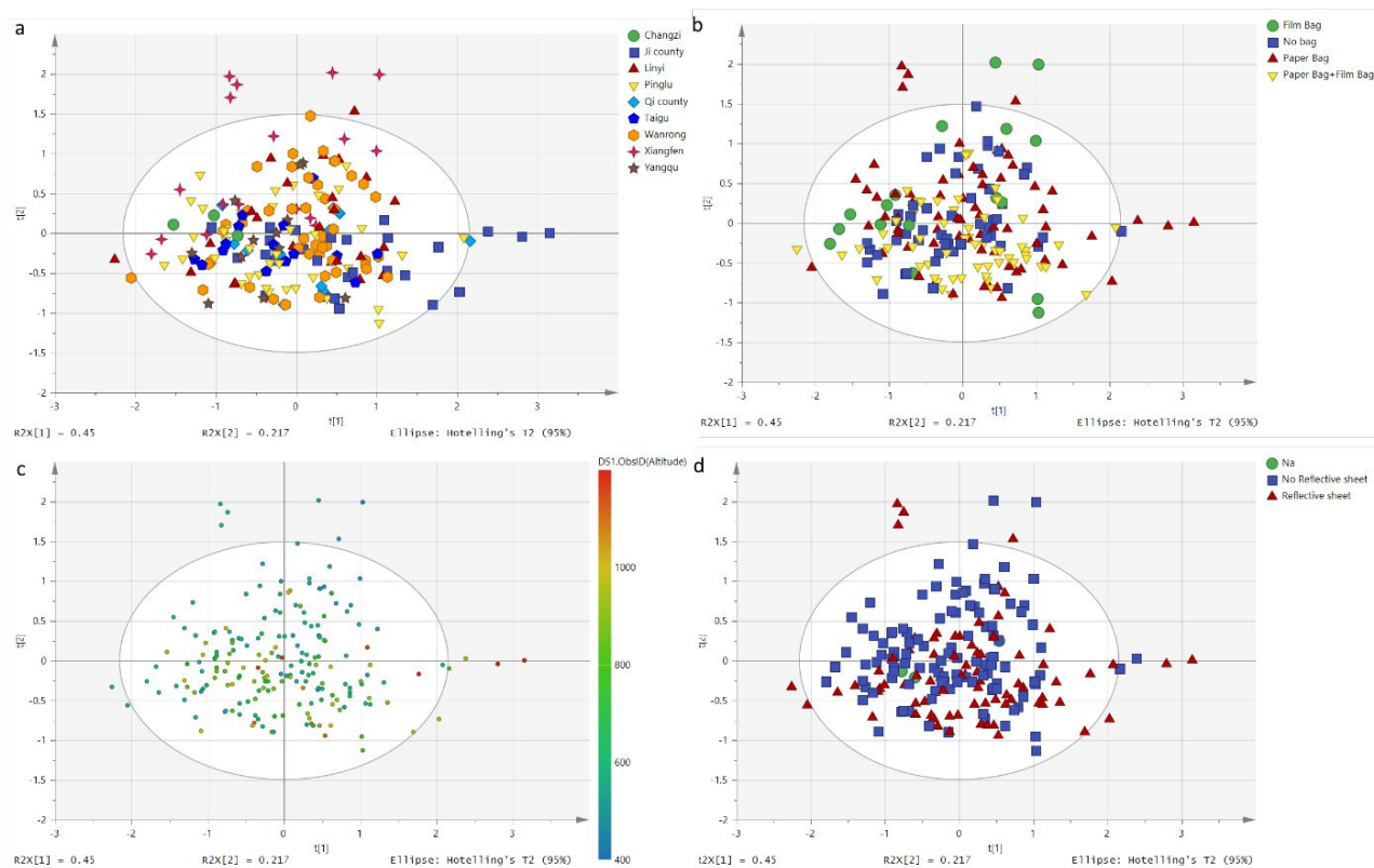
Figure S2. PCA score plots generated using binned data from full ^1\text{H} NMR spectra, based on different category strategies: location at the county level (a), bagging method (b), altitude (c), and reflective sheet condition (d).
