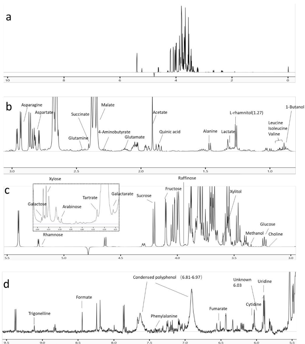
Figure S1. ^1\text{H} NMR spectrum of apples: Overview of the spectra (a); Spectrum from 0.5-3 ppm region (b); Spectrum from 3-5.6 ppm region (c); Spectrum from 5.6-10 ppm region (d)
