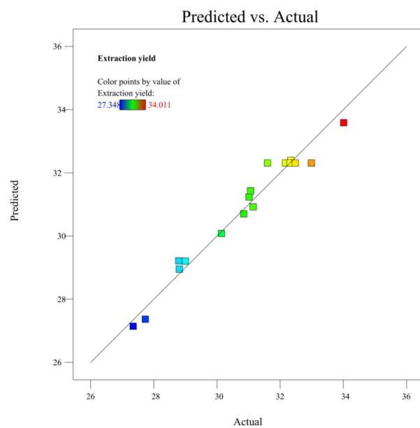
Supplementary Figure1 Correlation between the predicted and actual triterpenoids extraction
