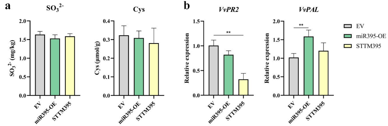
Supplementary Figure S3. Content of SO 3 2- , and Cys in grapes after transient transformation with miR395 (a). Relative expression level of pathogen response-related genes in grapes after transient transformation with miR395 (b). * p < 0.05, ** p < 0.01, *** p < 0.005.
