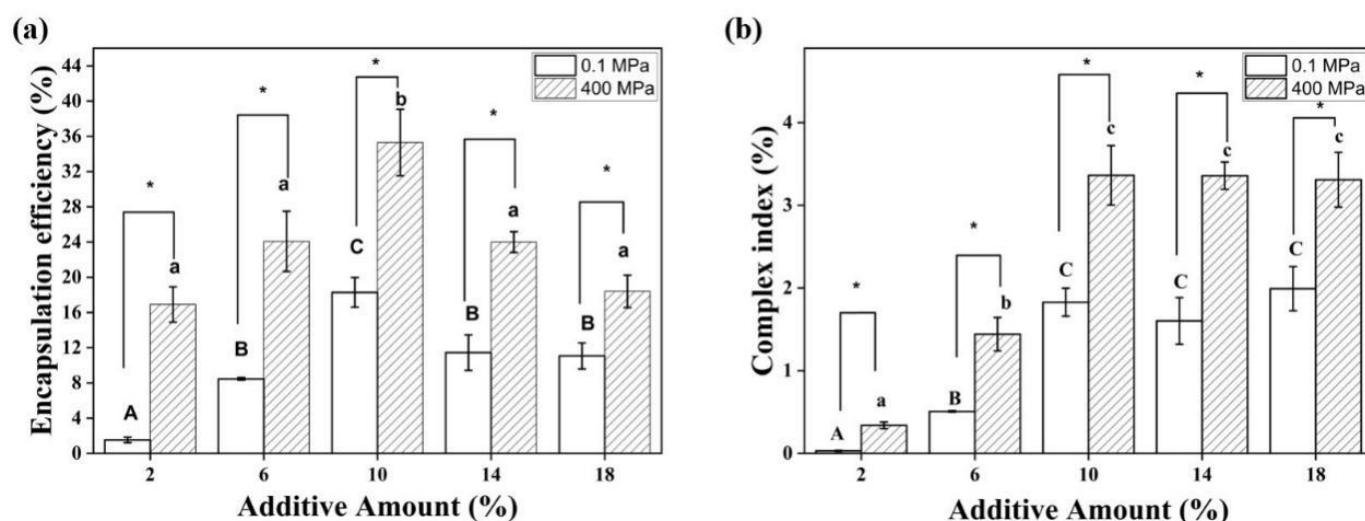
Supplementary Fig. S1. Effect of different LA amounts on the recombination efficiency (a) and binding rate (b) of corn starch-linoleic acid complex under ambient pressure (0.1 MPa) and high pressure (400 MPa/10 min)
