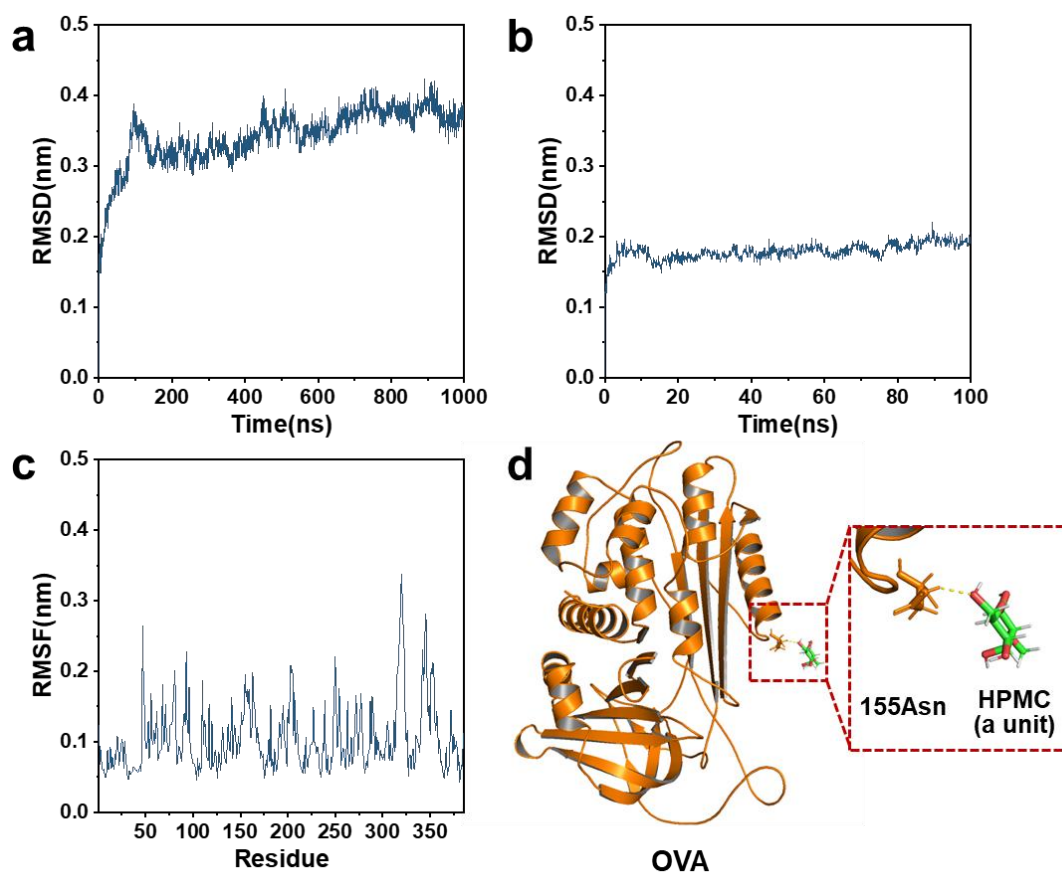
Supplementary Fig. S5 MD of the HPMC monomer and OVA. (a) RMSD of the protein under 307.15 K; (b) RMSD of the complex under 217.15 K; (c) RMSF of the residues in OVA under 217.15 K; (d) Visualization of HPMC monomer and OVA interactions.
