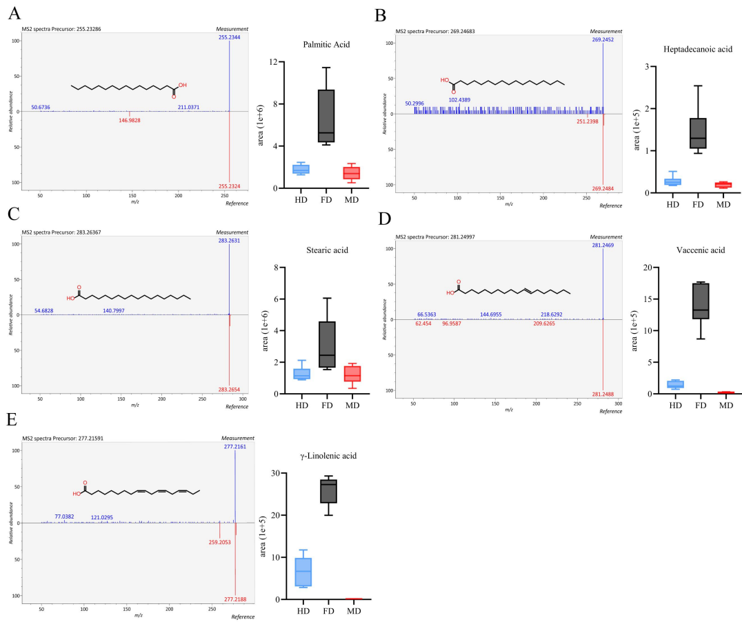
Supplementary figure S4. The free fatty acids markers in FD. The left part was mirror plots and chemical structures, and the right part was the box-plots. A) palmitic acid, B) heptadecanoic acid, C) stearic acid, D) vaccenic acid E) \gamma -linolenic acid.
