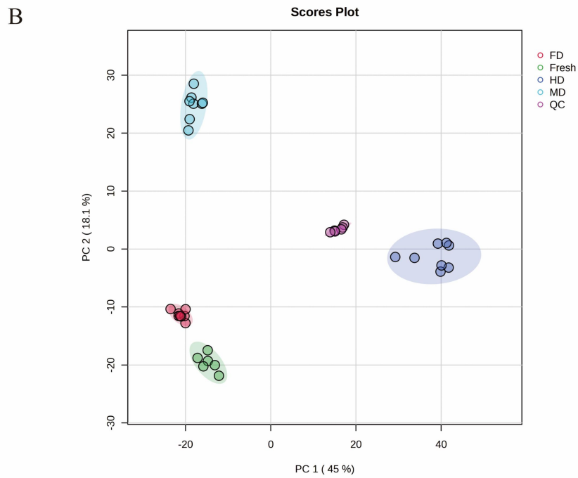
Supplementary figure S1. The total ion chromatograms of the QC (A) and PCA scores plot of samples and QC (B)
