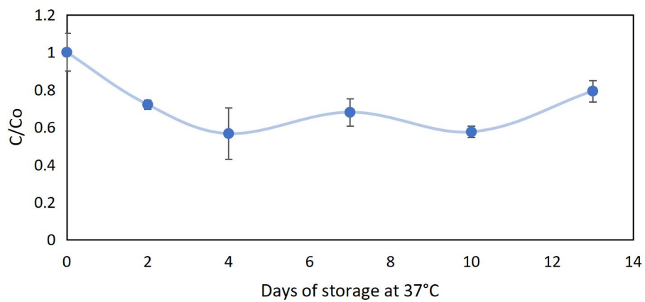
Figure S3: Trend in \beta -carotene dissolved in bulk sunflower oil degradation during storage in dark, n \geq 3
