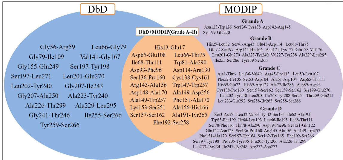
Supplemental Figure S1. The residue pairs forming potential disulfide bridges of carboxypeptidase A.
