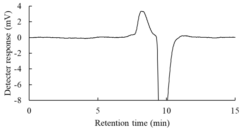
Fig. A.2 The elution profile of pectin from pitaya fruit peel.
