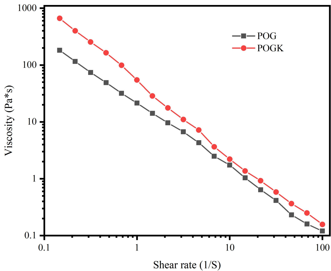
Figure S5. Viscosity measurement of POG and POGK hydrogels at 25 °C.
