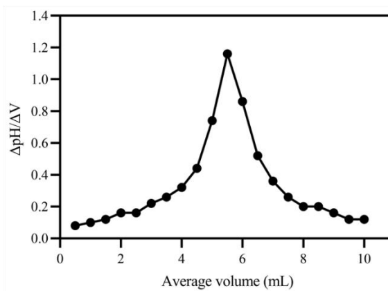
Figure S3. (a) The cartoon diagram of the titration procedure. (b) The first derivative of the hydroxylamine hydrochloride potentiometric titration.
