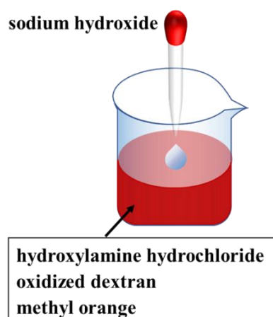
Figure S3. (a) The cartoon diagram of the titration procedure. (b) The first derivative of the hydroxylamine hydrochloride potentiometric titration.
