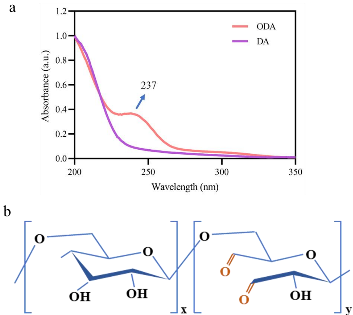
Figure S2. (a) The UV-vis spectrum of DA and ODA. (b) The chemical structure of ODA.
