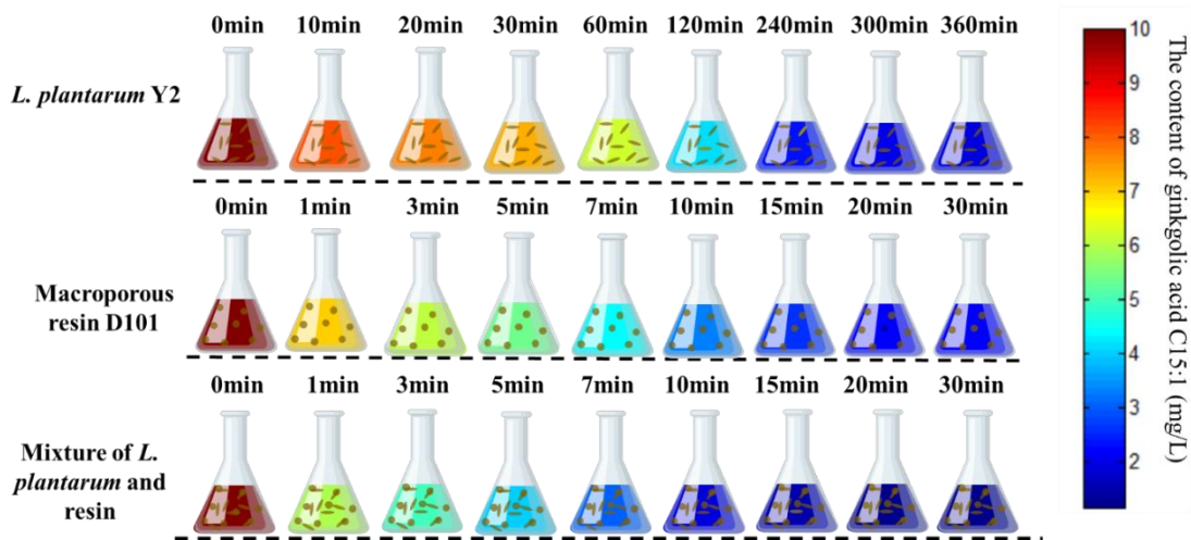
Supplementary Fig. 5. Changes in ginkgolic acid C15:1 content in the dispersions during absorption by L. plantarum Y2, macroporous resin D101, and their mixture as predicted by the PVSDM modeling.
