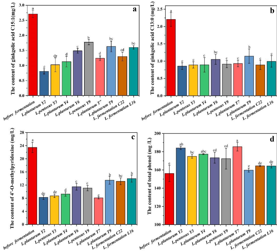
Supplementary Fig. 3. Comparison of the abilities of isolated microbial strains to remove toxins and enhance bioactives in ginkgo kernel juice after 48 h of fermentation. a: ginkgolic acid C15:1; b: ginkgolic acid C13:0; c: 4'-O-methylpyridoxine; d: total phenolics.
