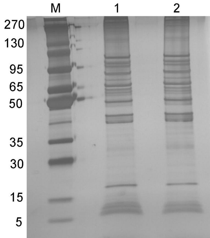
Supplementary Figure S2. SDS-PAGE analysis of whole cell surface proteins (lane 1) and proteins in the eluent (lane 2). The molecular masses (in kDa) of the standard proteins (lane M) were indicated on the left
