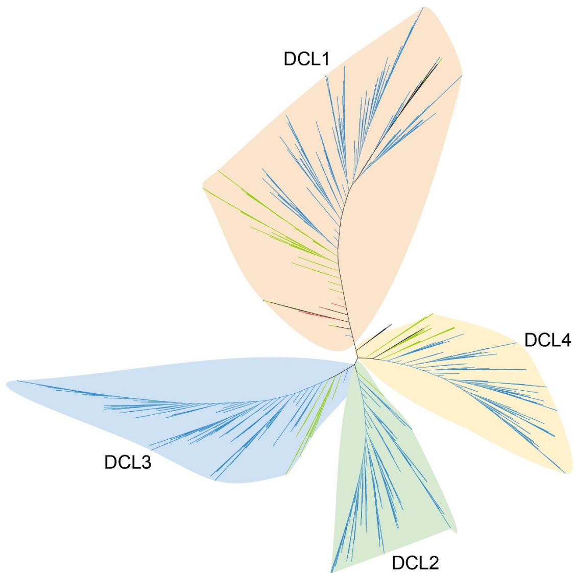
Supplementary Figure S1. The ML tree of DCLs identified with 1KP transcriptomic data. Branches are color-coded to denote different plant groups: black for rhodophytes, yellow for chlorophytes, red for charophytes, green for ferns and bryophytes, and blue for seed plants.
