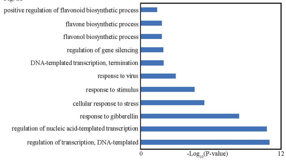
Figure S8. GO enrichment analysis of CG=>TG-related genes.
