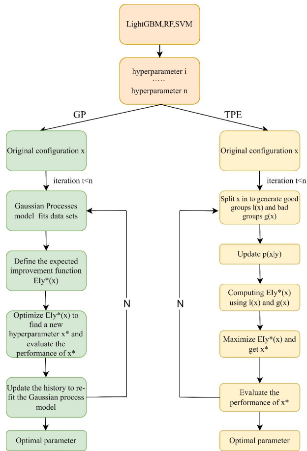
Supplementary Figure S2 Framework for model hyperparameter optimization
