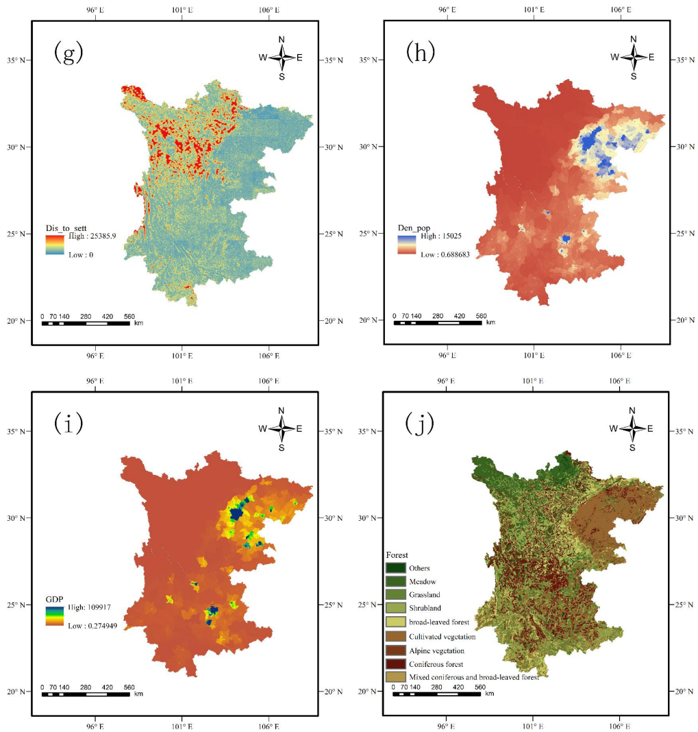
Supplementary Figure S1 Generalized plot of each factor: (a) elevation, (b) slope, (c) aspect, (d) topographic wetness index, (e) distance to nearest railway, (f) distance to nearest road, (g) distance to nearest settlement, (h) density of population, (i) GDP, (j) vegetation type.
