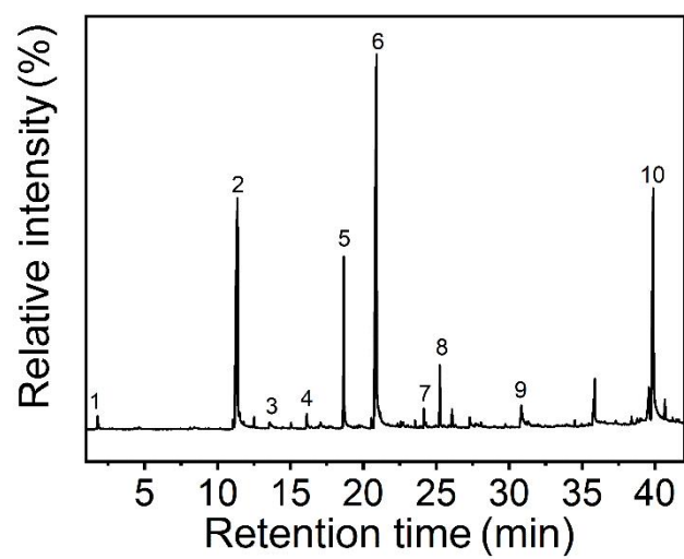
Fig. S8 Py-GC/MS spectra of EP/25% PA-DAD.
