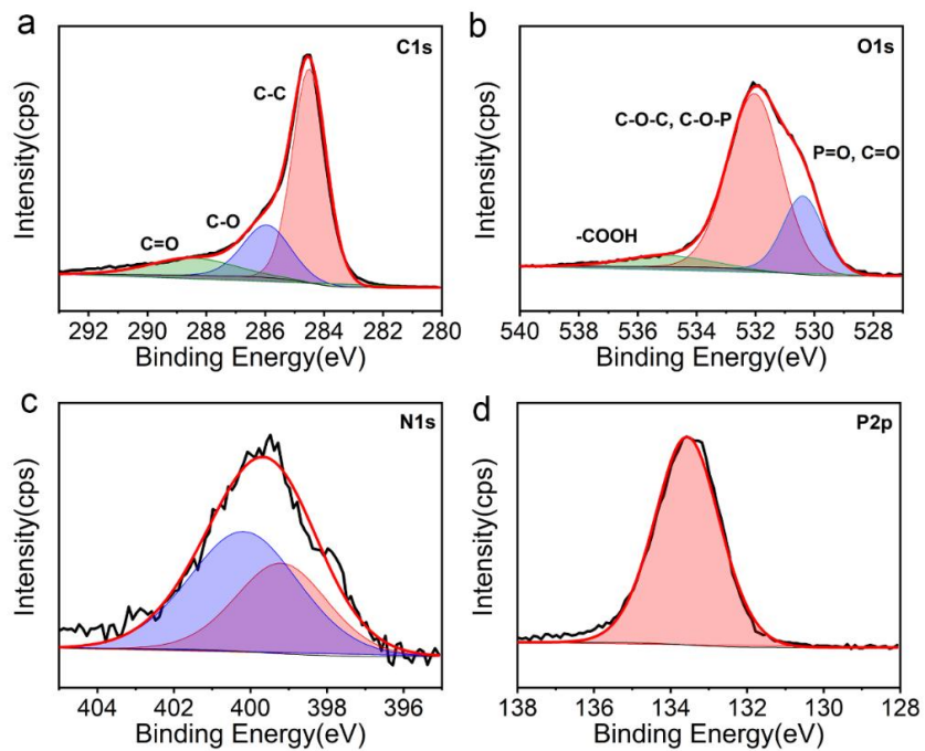
Fig. S6 (a) The C1s spectra of the composition of residual char; (b) The O1s spectra of the composition of residual char; (c) The N1s spectra of the composition of residual char; (d) The P2p spectra of the composition of residual char.
