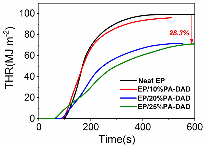
Fig. S4 The THR curves vs time for EP composites at a flux of 35 kW/m 2 .
