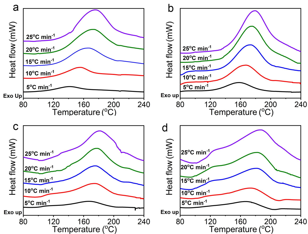
Fig. S2 The DSC curves of (a) neat EP, (b) EP/10% PA-DAD, (c) EP/20% PA-DAD, (d) EP/25% PA-DAD at different heating rates and the fitting curves based on Kissinger, and Ozawa methods for neat EP and EP composites.
