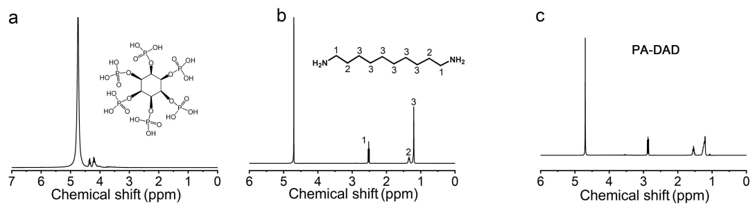
Fig. S1 ^1\text{H} NMR spectra of (a) PA, (b) DAD, and (c) PA-DAD.
