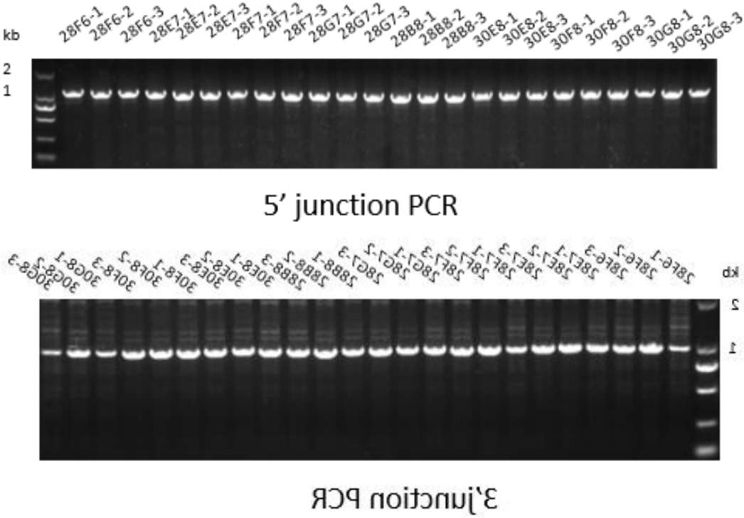
Fig. S5: Verification of correct integration of mcherry donor sequence with different heterotypic promoters. Target band size by 5' junction PCR was ~1.2 kb; target band size by 3' junction PCR was ~1 kb.
