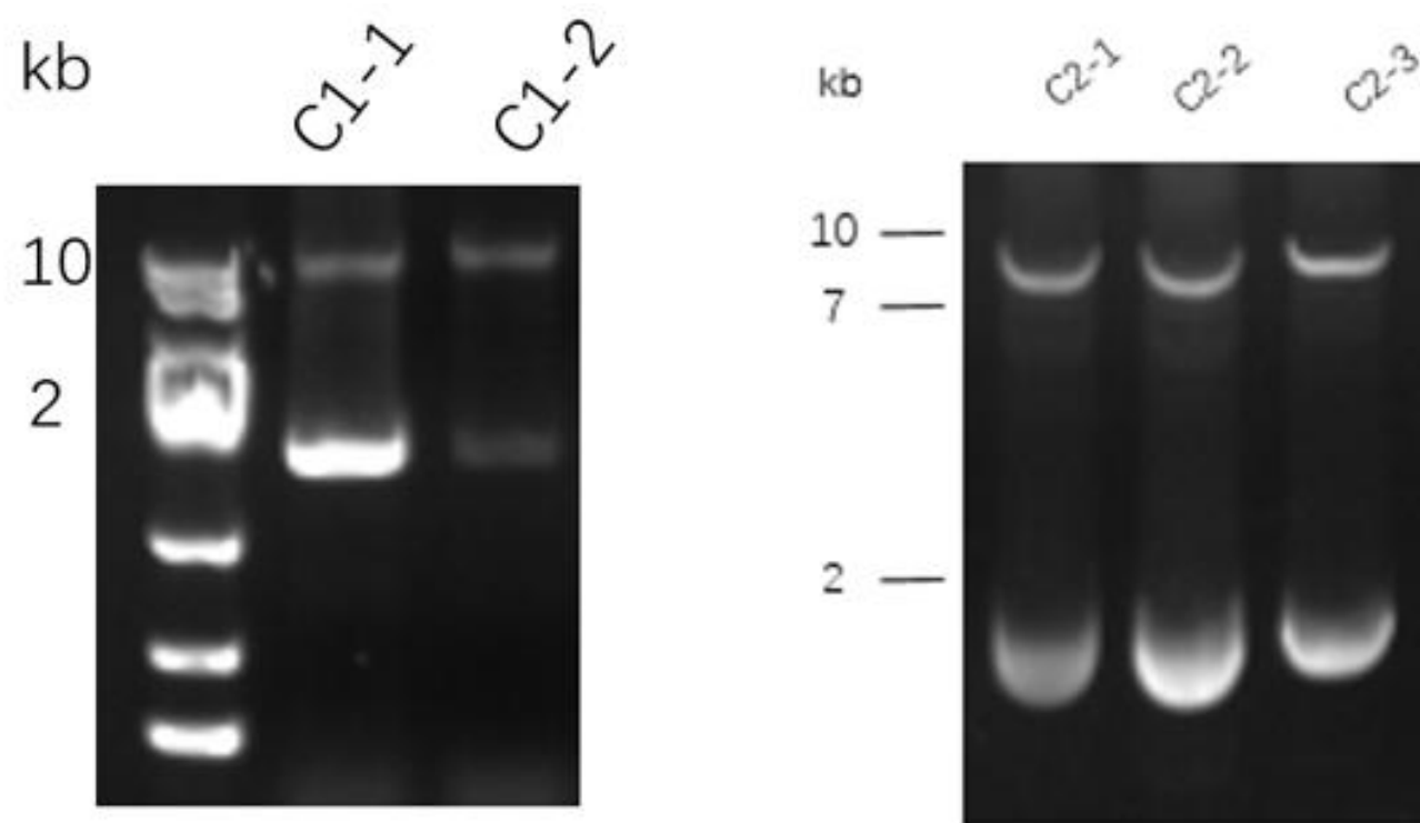
Fig. S9: Verification of correct integration of bsAb genes with different promoter combinations. Target band size by out-out PCR was ~12 kb for C1 and 9 kb for both C2.
