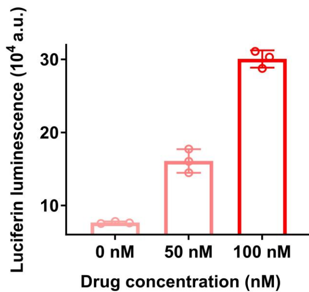
Figure S3. Application of P1-IN-Gluc for dose-dependent 3CL Pro inhibitor measurements. The major component of Paxlovid, nirmatrelvir (PF-07321332), was applied to the cell culture before signal readout.
