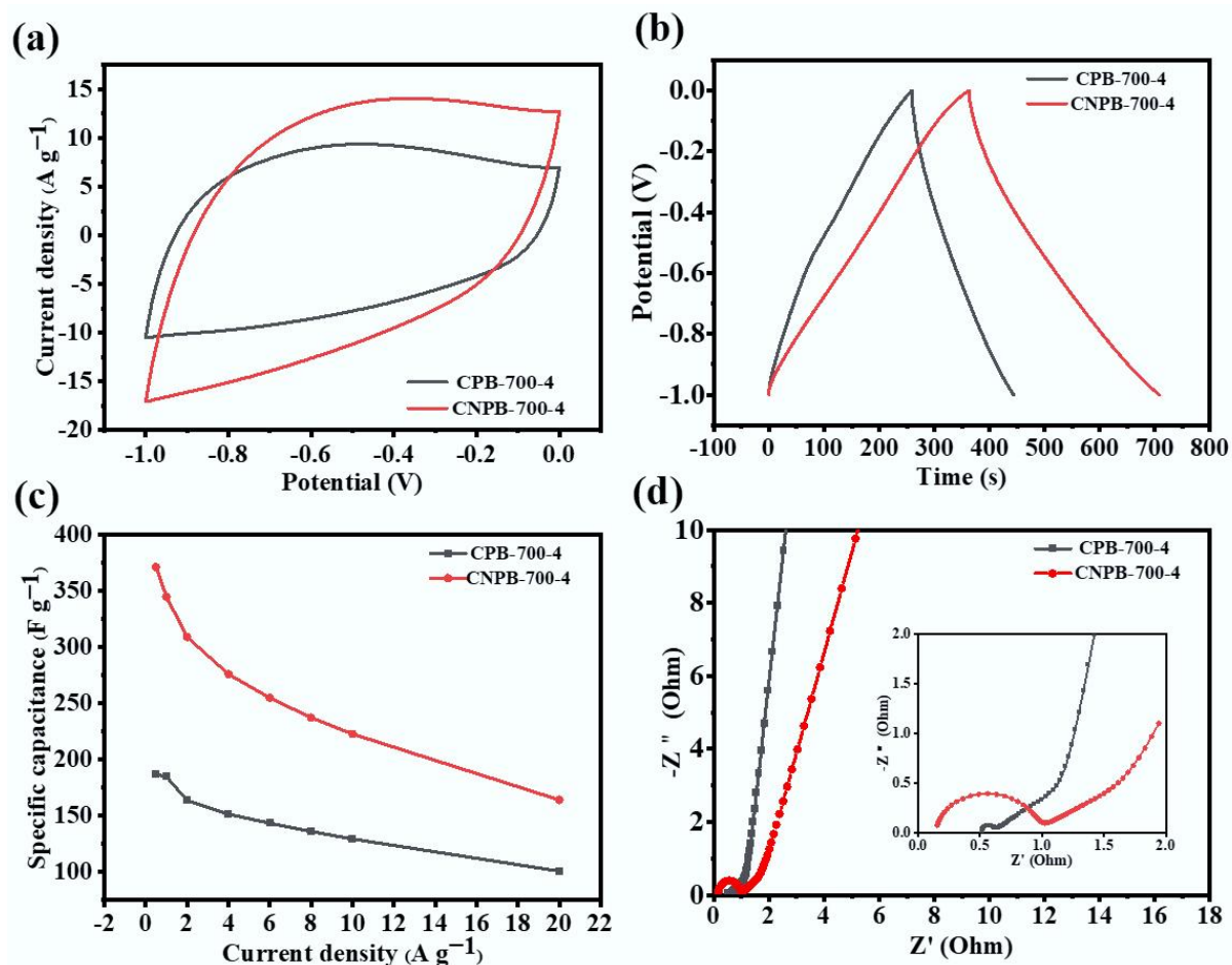
Fig. S1 (a) CV curves of CPB-700-4 and CNPB-700-4 at 50 \text{ mV s}^{-1} ; (b) GCD curves of CPB-700-4 and CNPB-700-4 at 1 \text{ A g}^{-1} ; (c) specific capacitance of CPB-700-4 and CNPB-700-4; (d) impedance profiles of CPB-700-4 and CNPB-700-4.
