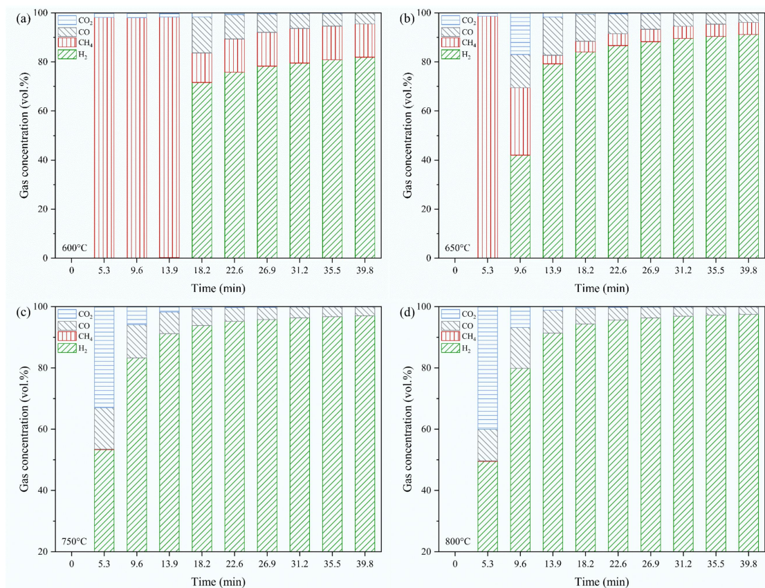
Supplementary Fig. S3 The gas concentration of H 2 , CH 4 , CO, and CO 2 under the catalysis of S3 catalyst at (a) 600 °C; (b) 650 °C; (c) 750 °C; (d) 800 °C.
