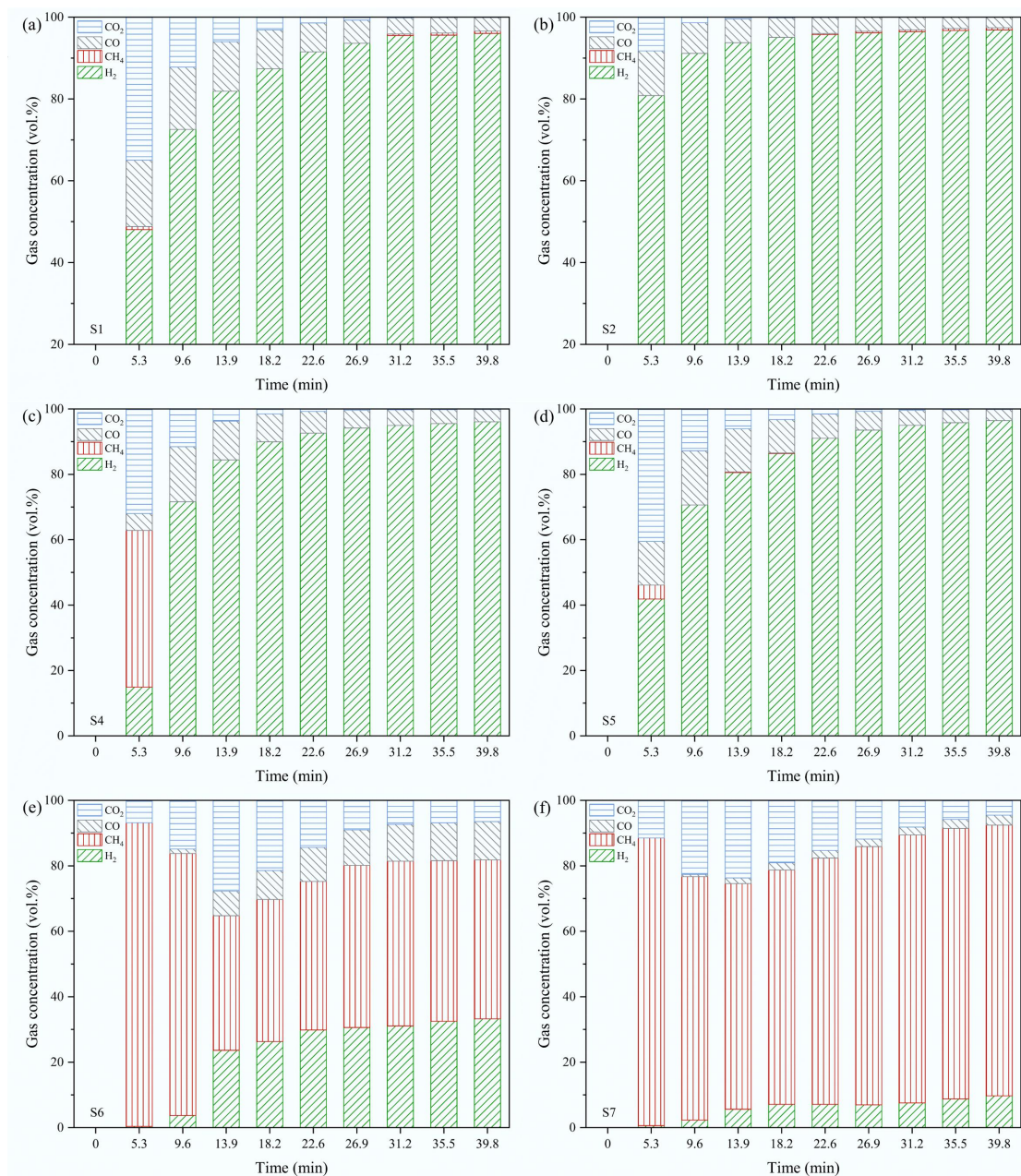
Supplementary Fig. S2 The gas concentration of H 2 , CH 4 , CO, and CO 2 under the catalysis of S3 (a) S1; (b) S2; (c) S4; (d)
