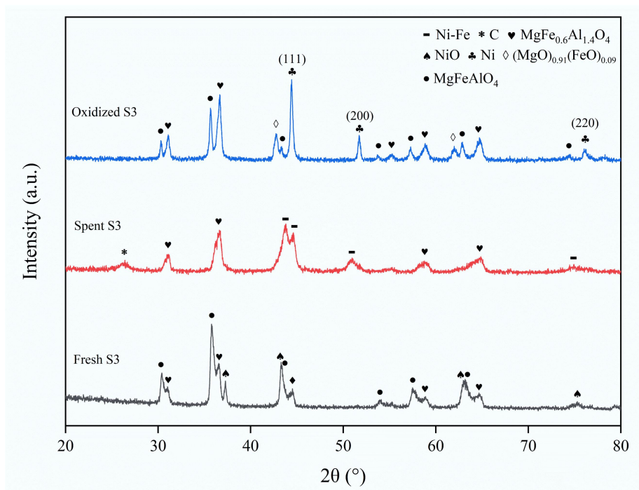
Supplementary Fig. S1 XRD patterns of the reacted S3 sample in fresh, spent, and \text{CO}_2 oxidized states.
