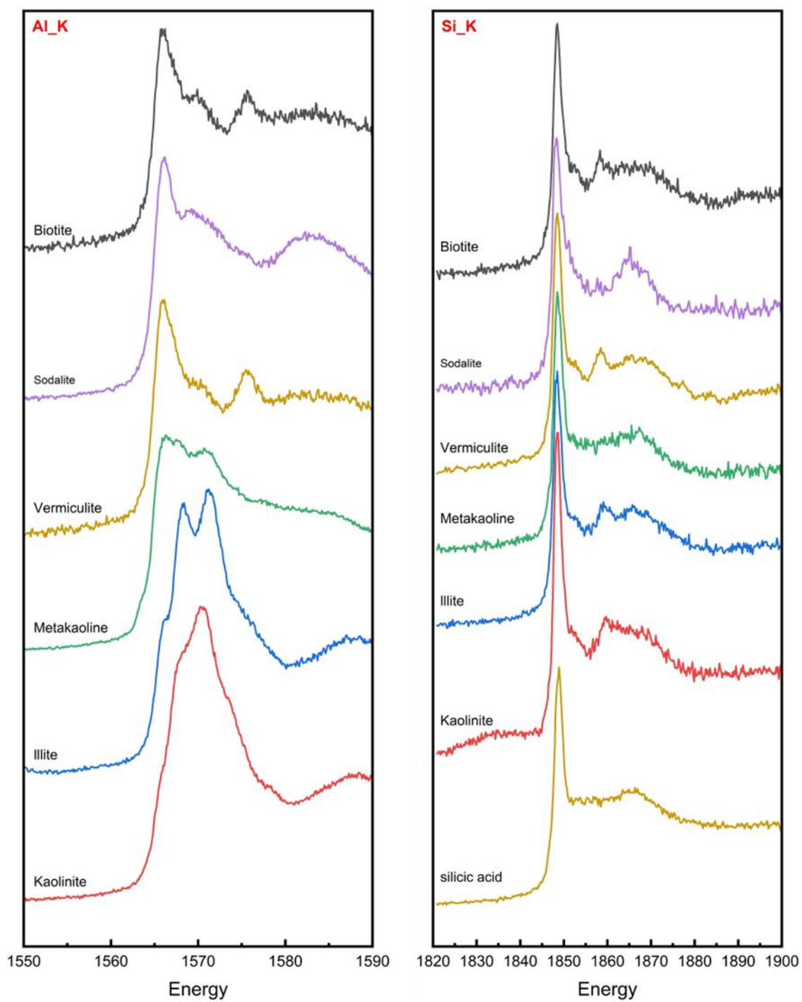
Supplementary Fig. S2. Al and Si K edge XAFS spectra of representative Al and Si standards.
