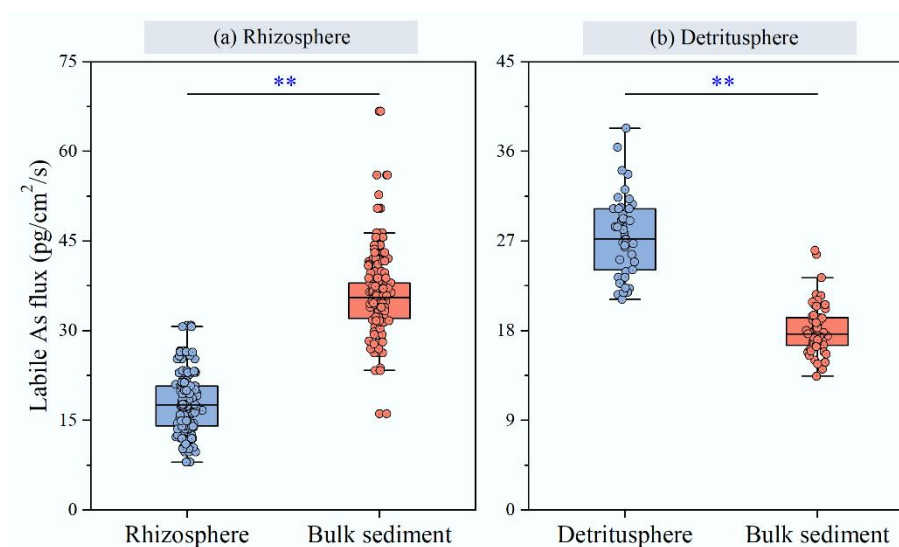
Supplementary Fig. S7 Labile As fluxes in the rhizosphere of rhizosphere (a) and detritosphere (b), respectively. (Significance levels: ** p < 0.01 ).
