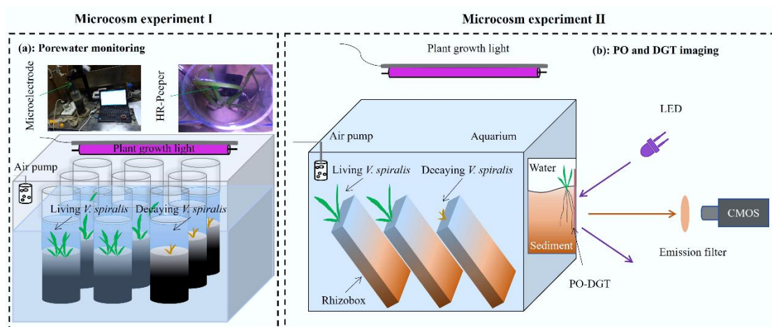
Supplementary Fig. S1 Microcosm experimental setup. (a) Microcosm experiment I containing Perspex tubes for monitoring the variations in porewater chemistry with root growth and root degradation. (b) Microcosm experiment II containing rhizoboxes for imaging the distribution of O 2 and labile As.
