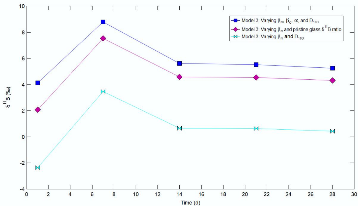
Supplementary Fig. S4. Residuals from applying Model 3 to the ^{10}B -ISG solution renewal experiment solution \delta^{11}B values. Fits were obtained by fitting the non-renewal experiments first using Model 3, holding these parameters constant, and then applying these rigid models to the solution renewal experiment data.
