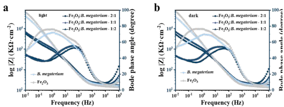
Figure S15. The \text{Fe}_2\text{O}_3/B. megaterium biofilm was conducive to electron transfer. Bode plot of before and after interaction between B. megaterium and \text{Fe}_2\text{O}_3 in the light (a) and dark (b).
