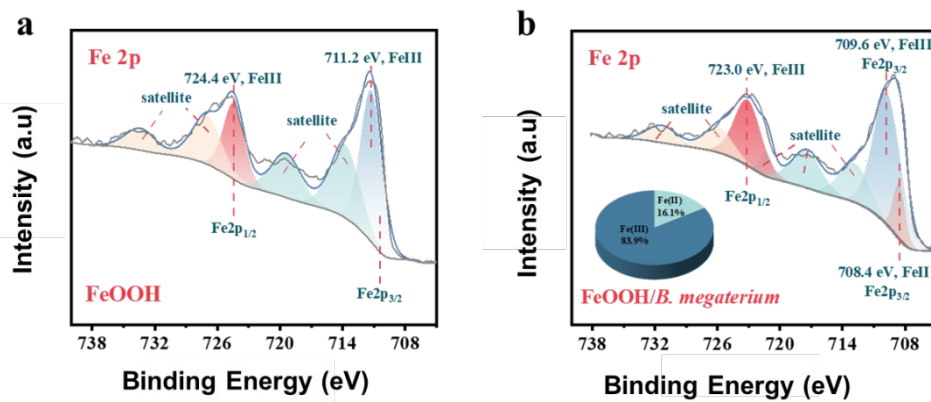
Figure S12. Fe 2p XPS spectra of FeOOH and FeOOH/ B. megaterium
