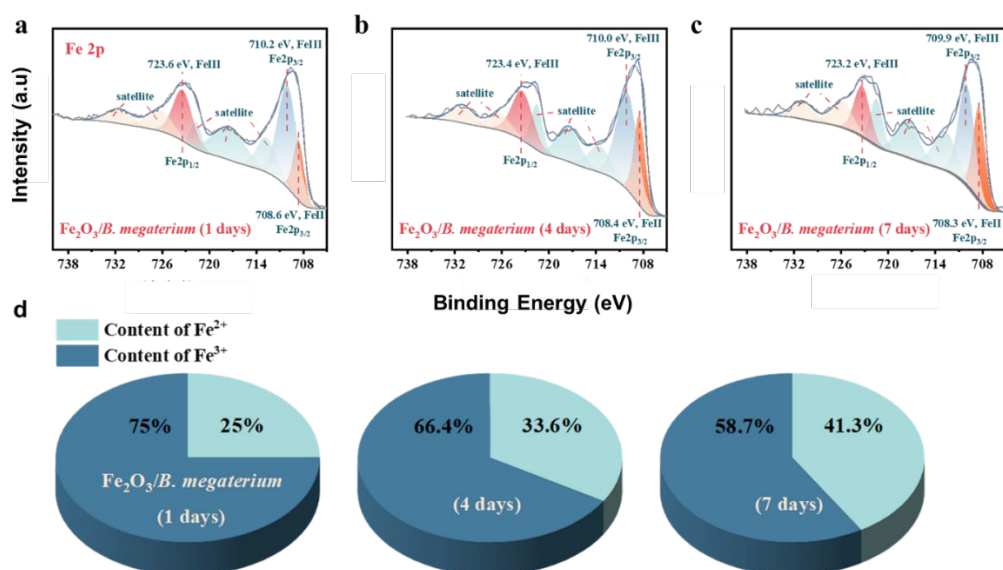
Figure S11. \text{Fe}_2\text{O}_3/\text{B. megaterium} composites Fe 2p XPS spectra and magnified region plots at different incubation times 1 day (a), 4 days (b), 7 days (c); Relative contents of Fe(III) and Fe(II) in \text{Fe}_2\text{O}_3/\text{B. megaterium} at different incubation times (d)
