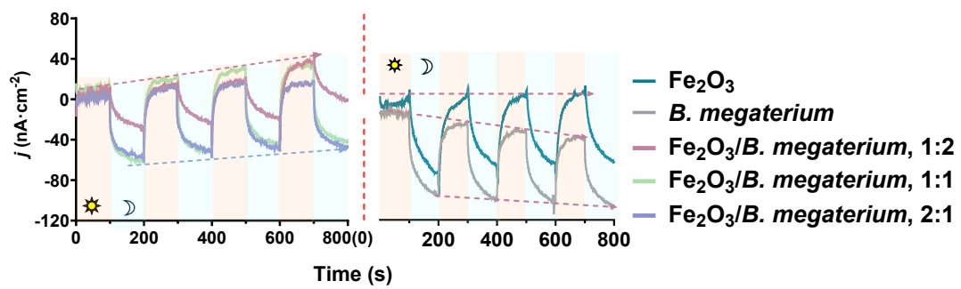
Figure S2. This \text{Fe}_2\text{O}_3 - B. megaterium system showed electro-charging and discharging processes under alternating light and dark conditions.
